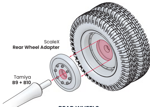
REAR WHEELS
