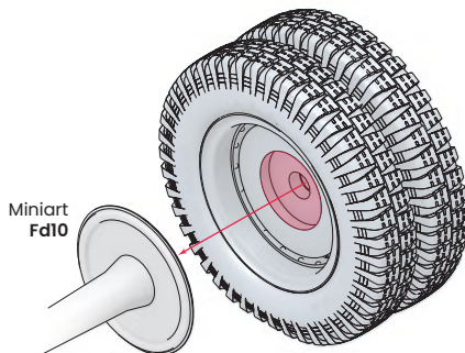
REAR WHEELS
