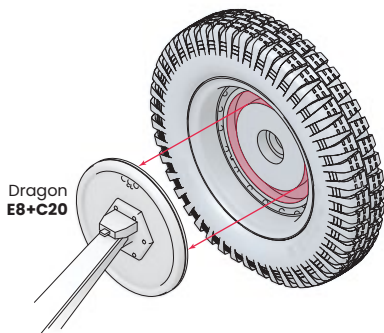
FRONT WHEELS
