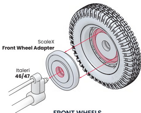
FRONT WHEELS
