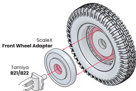
FRONT WHEELS
