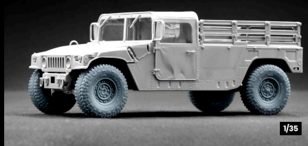
HMMWV MT/R 24-bolt Wheel Set (Ordinary) ScaleX Universal Mounting
